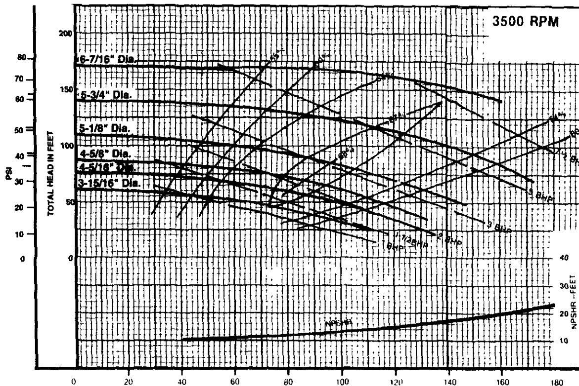
Performance Chart - 3500RPM
