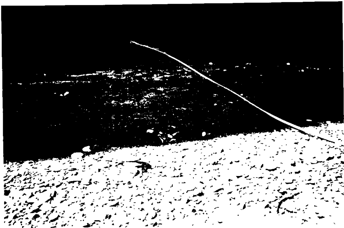
PHOTO ONE- Point of diversion in South Fork of Payette River. A portion of the approximately 175' of 2" PVC to pump on upper portion of river bank is shown.
