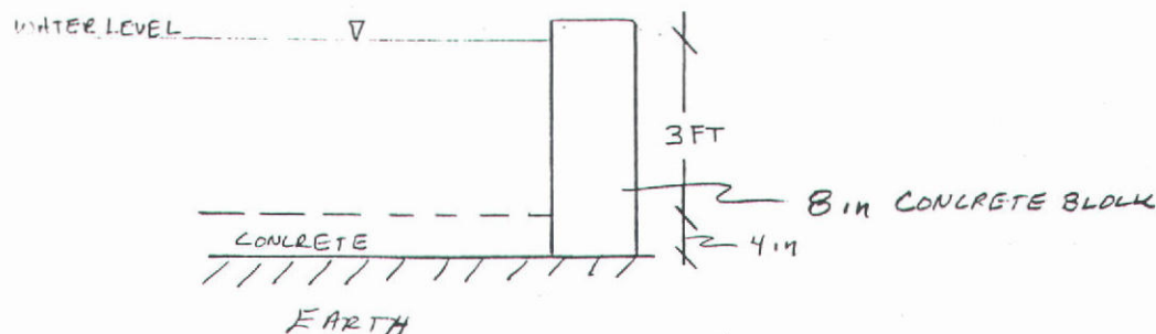
CROSSSECTION
