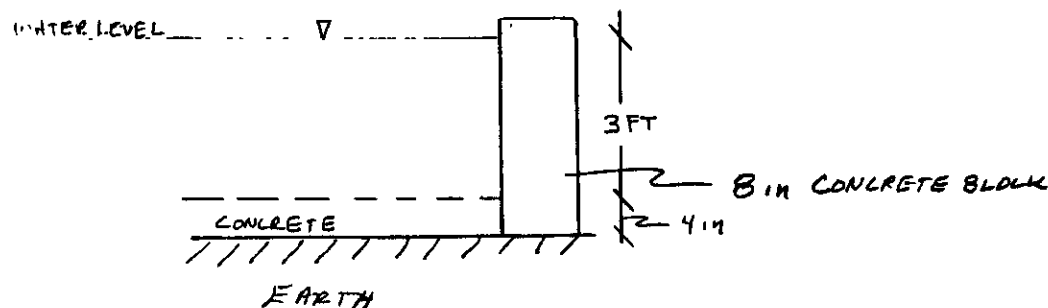
CROSSSECTION
