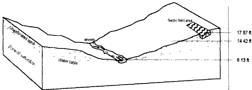
Cross-section at Truman-Tunie property
