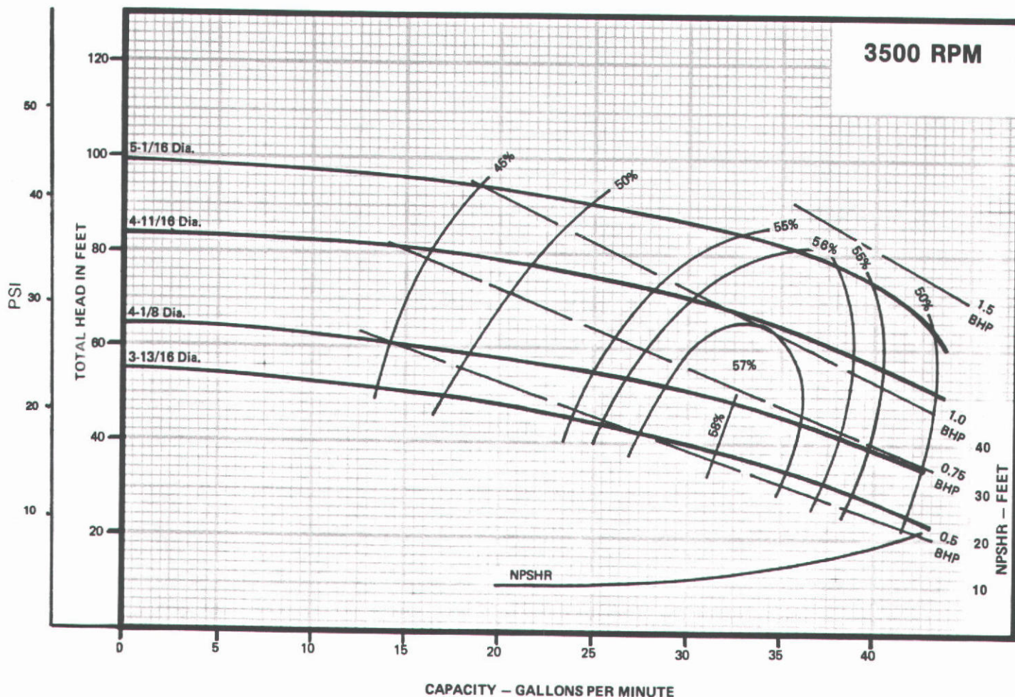
Performance Chart - 3500 RPM
