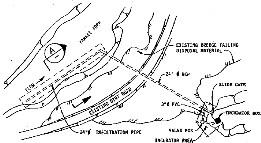
POND SERIES 4 INTAKE FACILITIES PLAN
