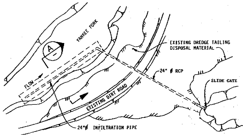
POND SERIES 4 INTAKE FACILITIES PLAN
