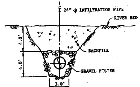
SECTION A
