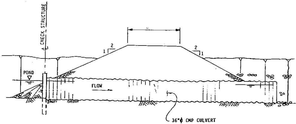
SECTION A
