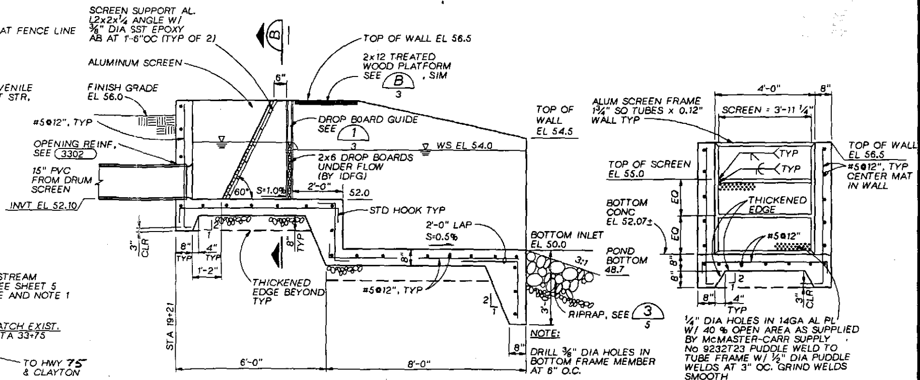
SECTION (A) 1/2"=1'-0"
