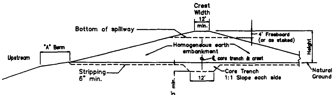
CROSS-SECTION (Bottom of Drainage)
