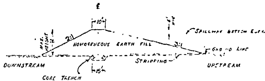
TYPICAL CROSS-SECTION
