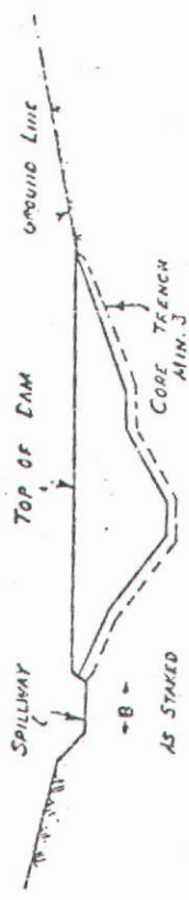
TYPICAL PROFILE NTS
