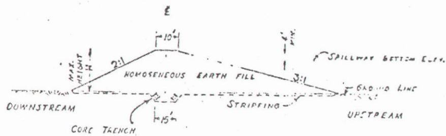
TYPICAL CROSS-SECTION
