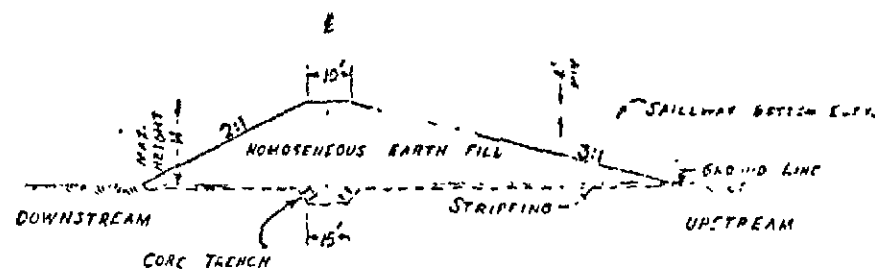
TYPICAL CROSS-SECTION N.T.
