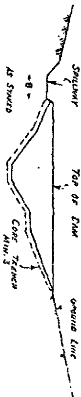
TYPICAL PROFILE
