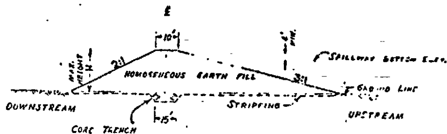
TYPICAL CROSS-SECTION
