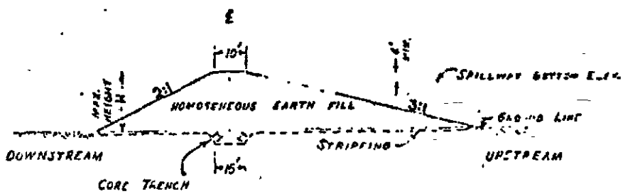
TYPICAL CROSS-SECTION
