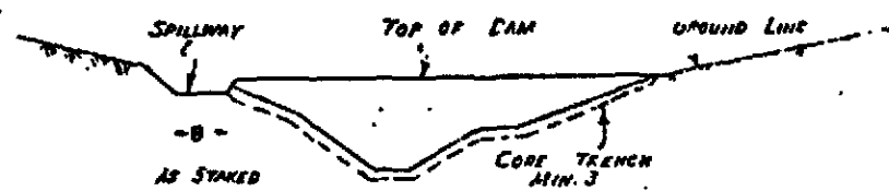
TYPICAL PROFILE
