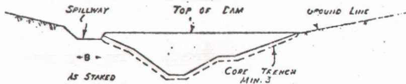
TYPICAL PROFILE
