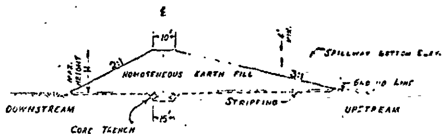
TYPICAL CROSS-SECTION
