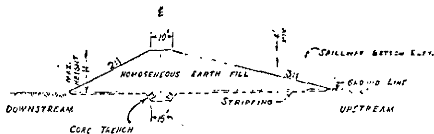
TYPICAL CROSS-SECTION N o 3
