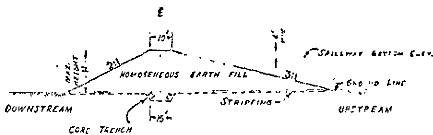
TYPICAL CROSS-SECTION N-3
