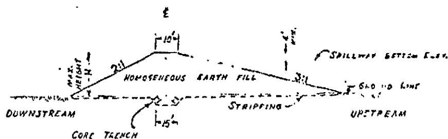
TYPICAL CROSS-SECTION
