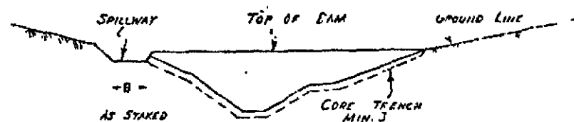
TYPICAL PROFILE
