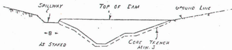
TYPICAL PROFILE
