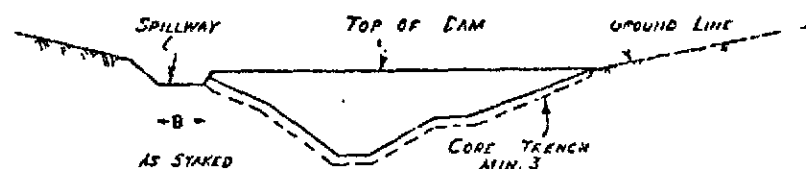
TYPICAL PROFILE 1/1.
