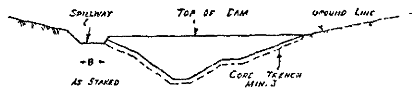
TYPICAL PROFILE HT.
