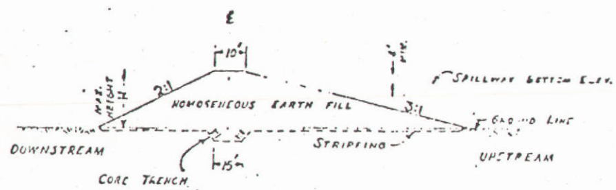
TYPICAL CROSS-SECTION N-S
