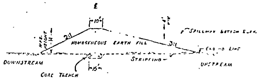
TYPICAL CROSS-SECTION
