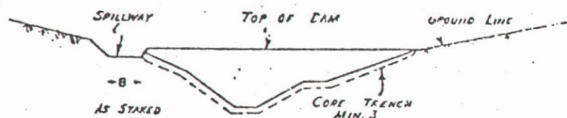
TYPICAL PROFILE HT.
