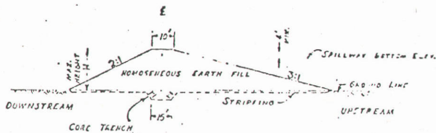
TYPICAL CROSS-SECTION
