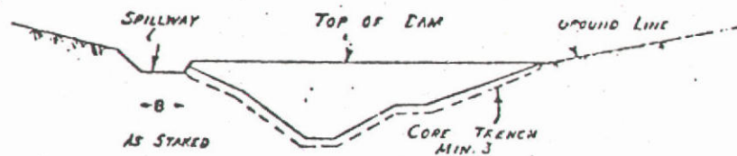
TYPICAL PROFILE
