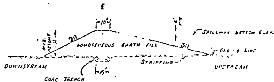
TYPICAL CROSS-SECTION
