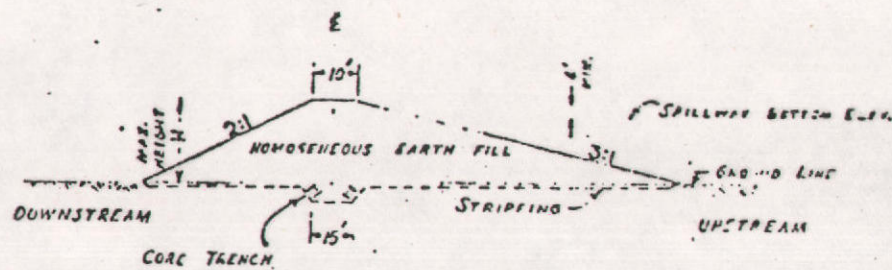
TYPICAL CROSS-SECTION
