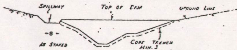
TYPICAL PROFILE
