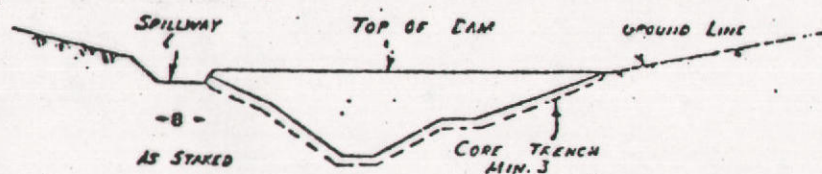
TYPICAL PROFILE
