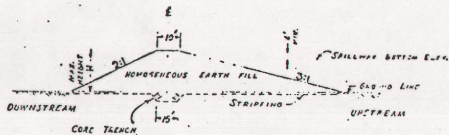
TYPICAL CROSS-SECTION
