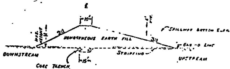
TYPICAL CROSS-SECTION
