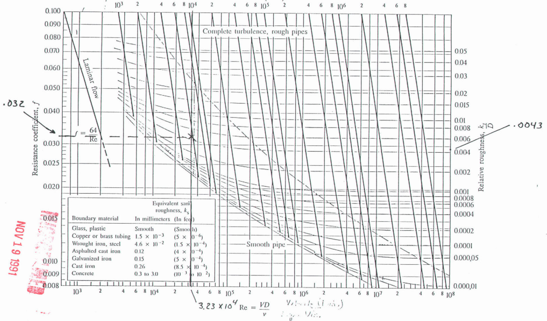
MOODY DIAGRAM
