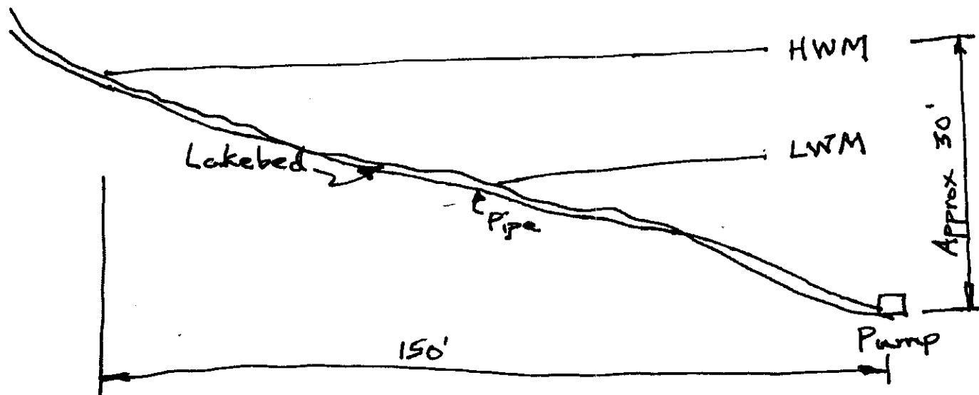
Elevation View
