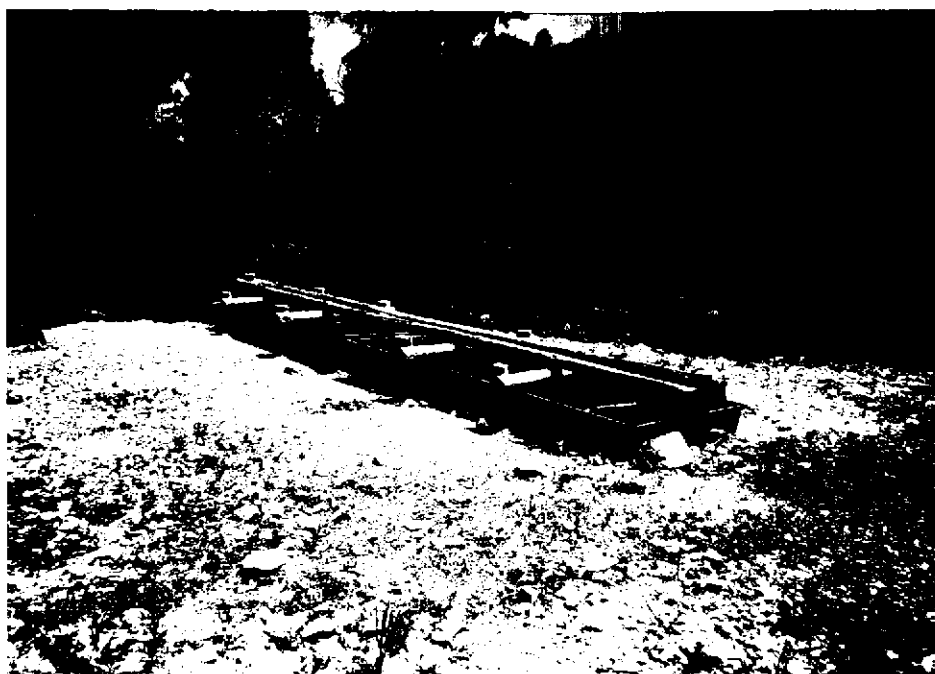
Fig. 3 - Stockwater trough at place of use.
