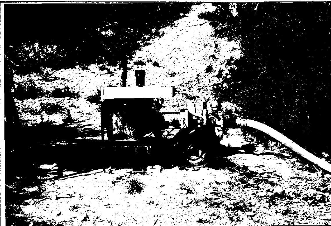
VIEW OF PORTABLE PUMP SYSTEM
