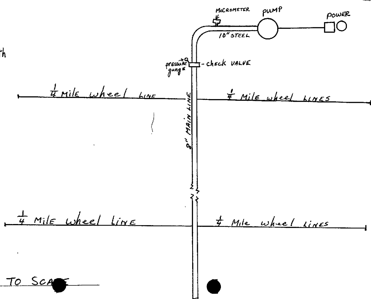
Diagram of System County Road
