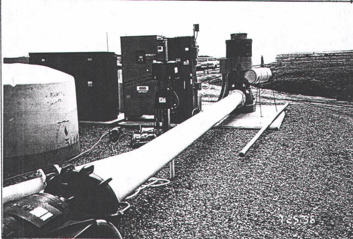
VIEW OF POINT OF DIVERSION WELL + PUMP
