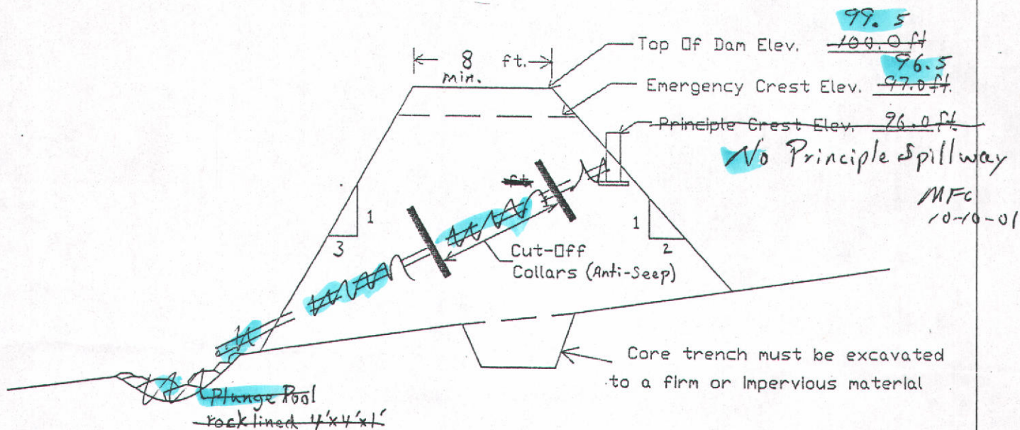
Dam X-Sec At Centerline
