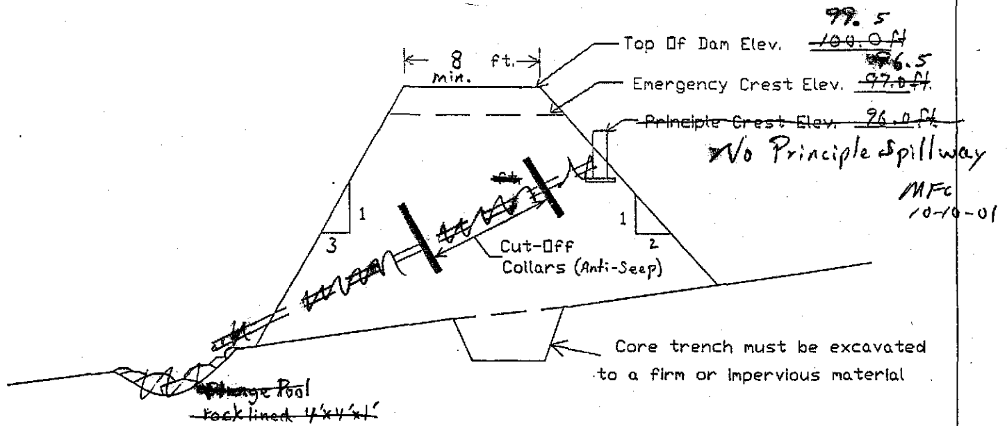
Dam X-Sec At Centerline
