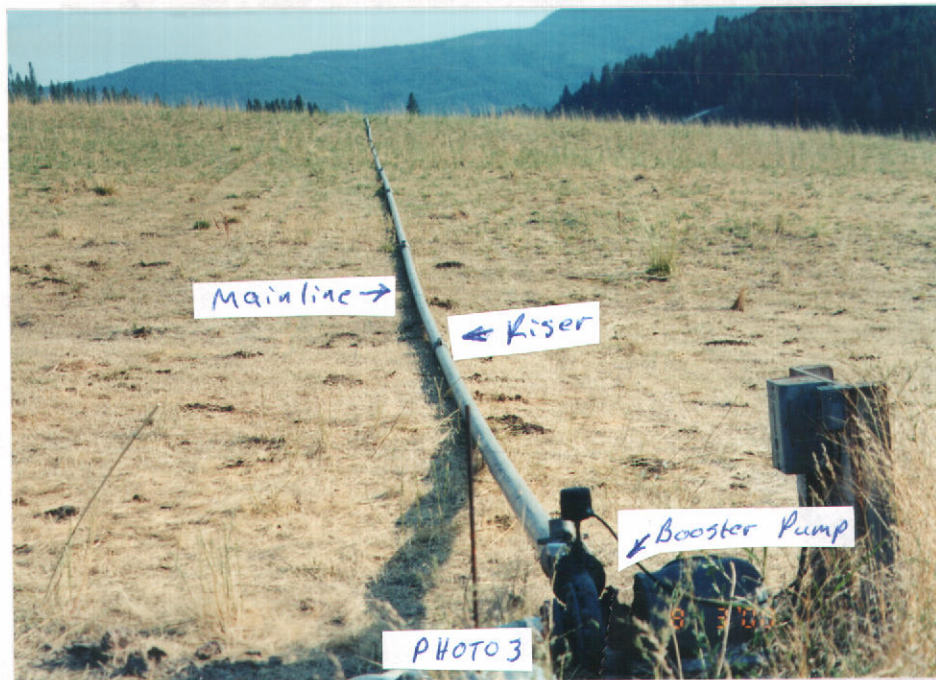
Photo 3. Showing main line to pasture from well and booster pump.
