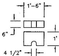
Saddle Block
