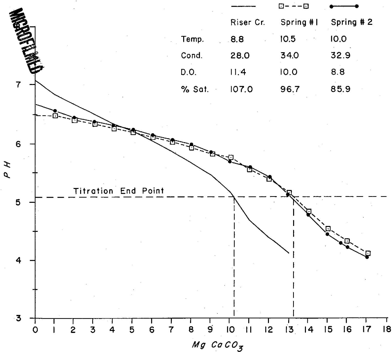
Alkalinity Titration Curve For Riser Creek And Tributary Springs.
