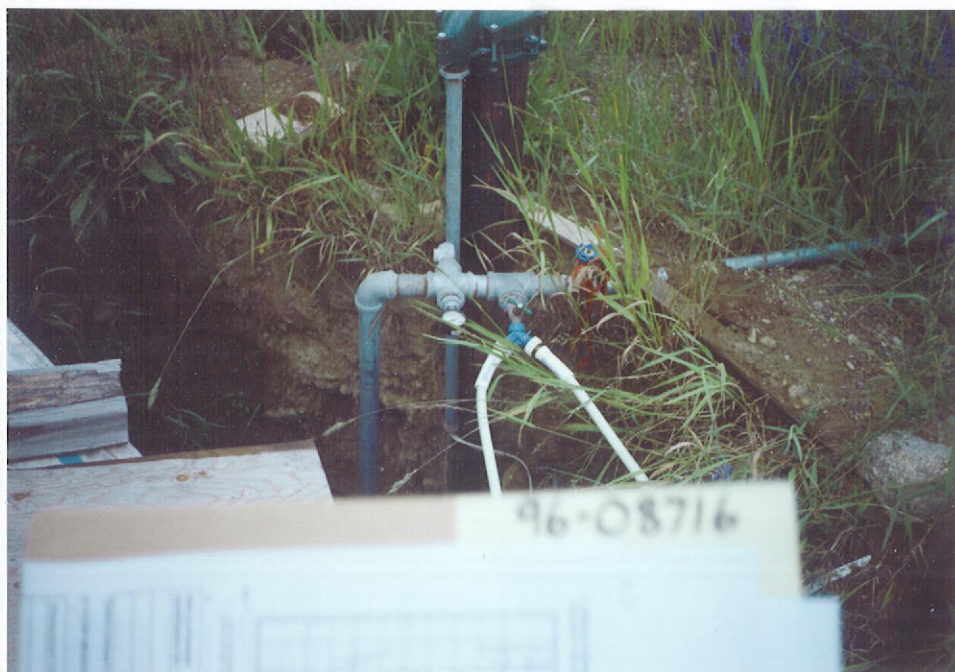
← GERALD WOODS WELL WITH GARDEN HOSE SET-UP. WELL IS EXPOSED.
