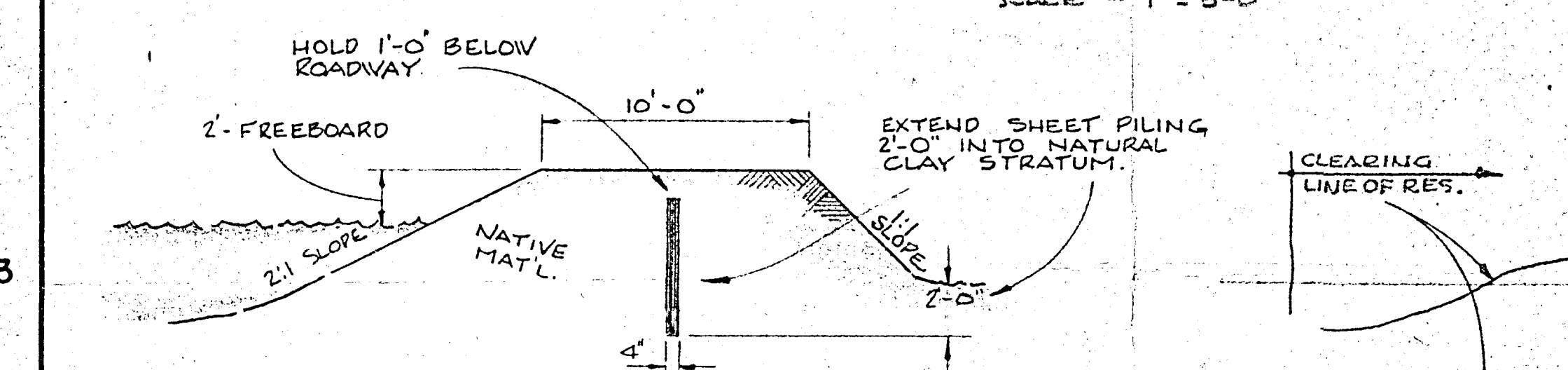
RESERVOIR DIKE TYPICAL CROSS SECTION ALTERNATE #2 SCALE - 1" = 5'-0"
