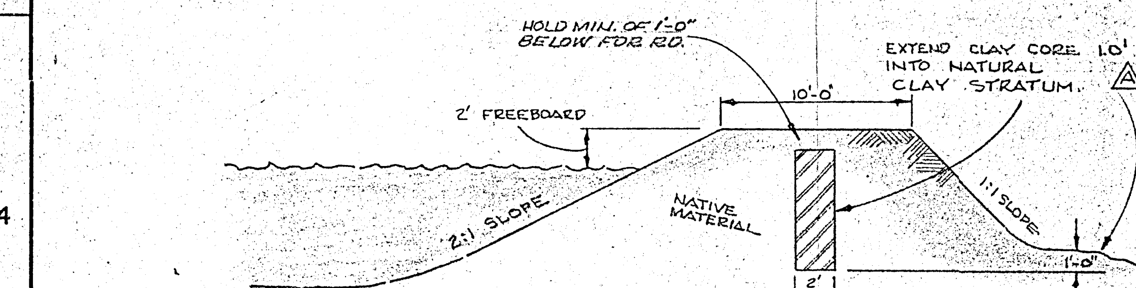
RESERVOIR DIKE TYPICAL CROSS SECTION ALTERNATE #1 SCALE - 1" = 5'-0"
