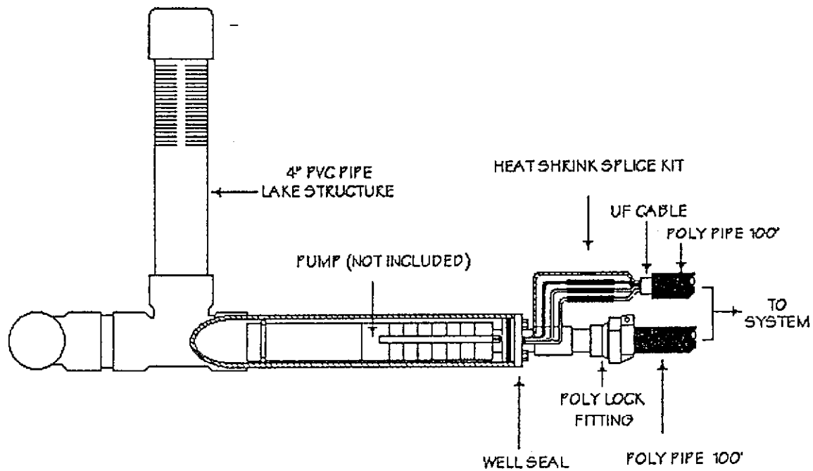
SIDE VIEW
