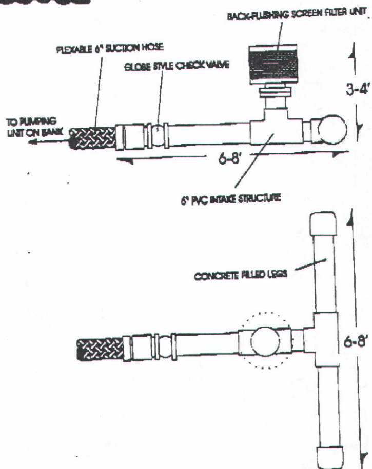
INSTALLATION DRAWING
