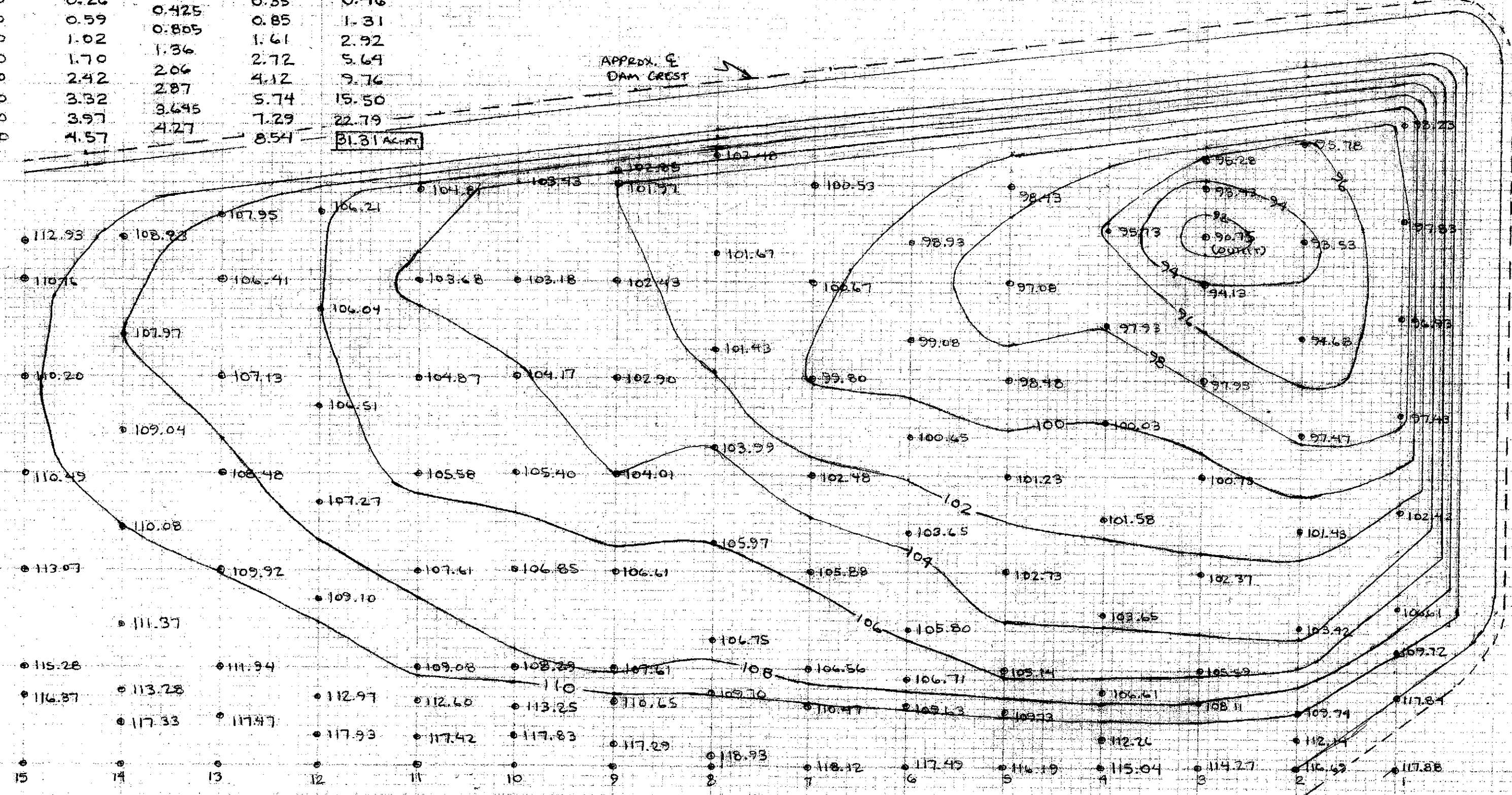
SCALE: 1" = 50 FT WIGGINS DAM NO 3 (D67-7931) RESERVOIR CONTOUR MAP
