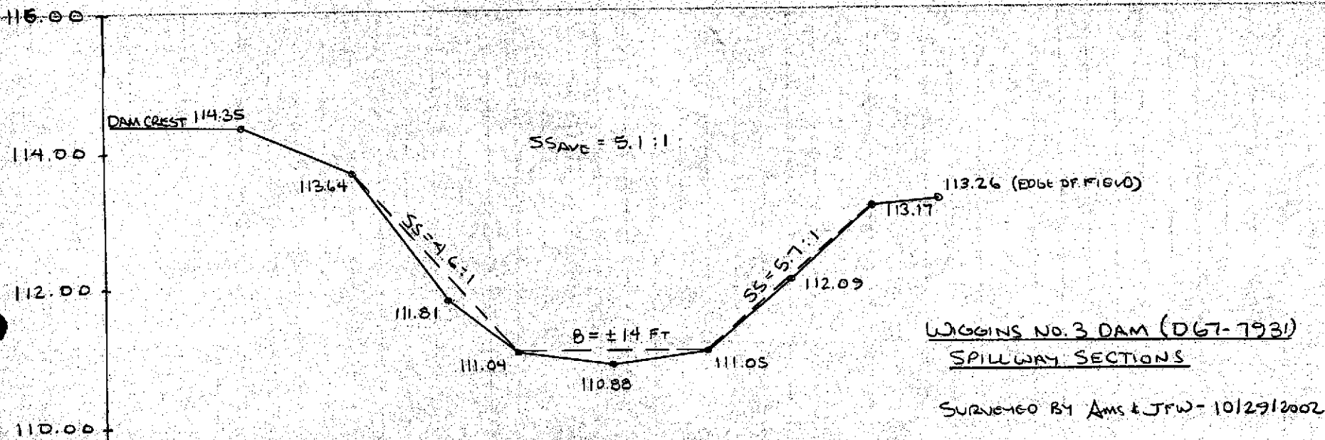
SPILLWAY X-SECTION TAKEN @ 0+50 ON PROFILE
