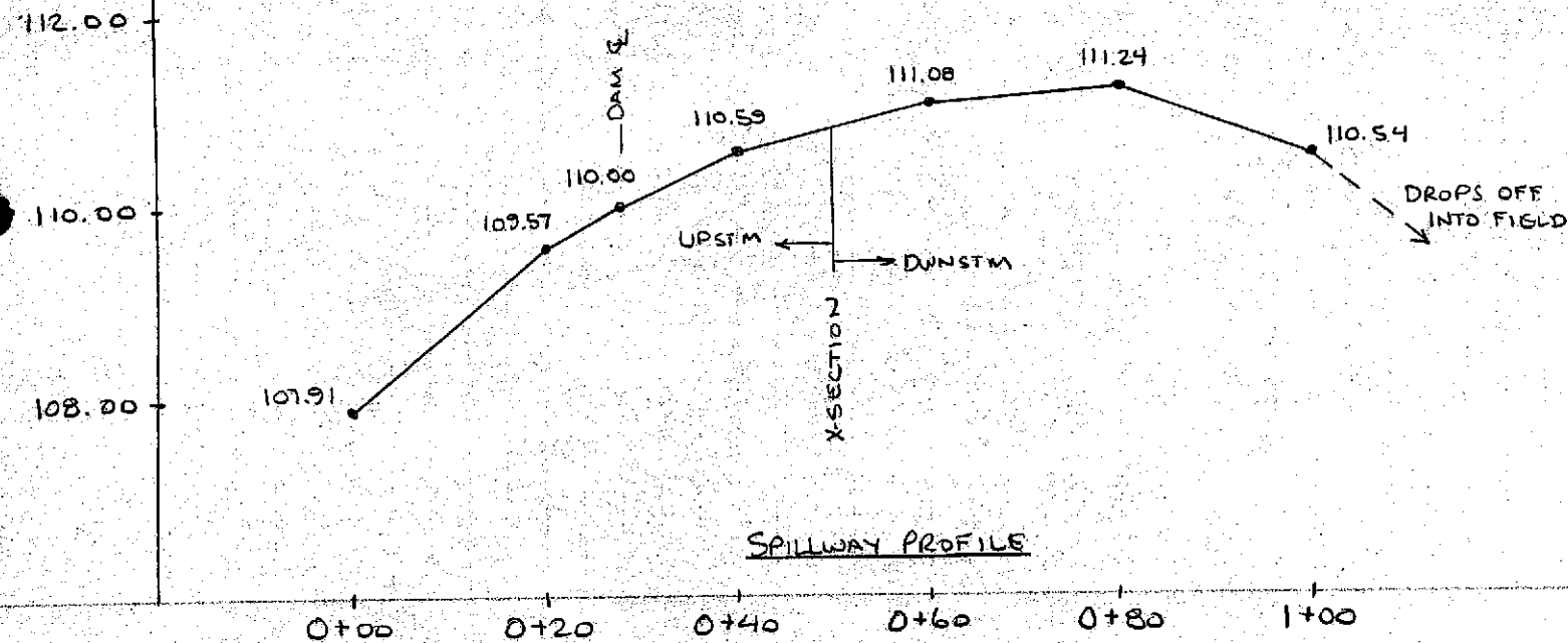
SPILLWAY X-SECTION TAKEN @ 0+50 ON PROFILE
