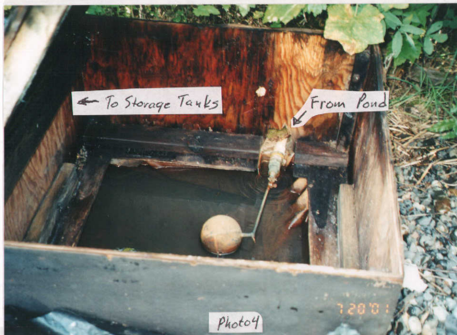
Photo 4. Showing float valve on the inside of control box.
