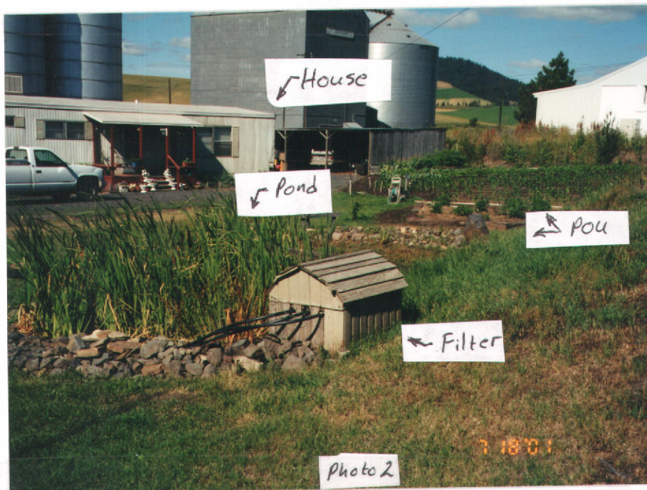
Photo 2. Showing recirculation filter, pond and a portion of the Place of Use.
