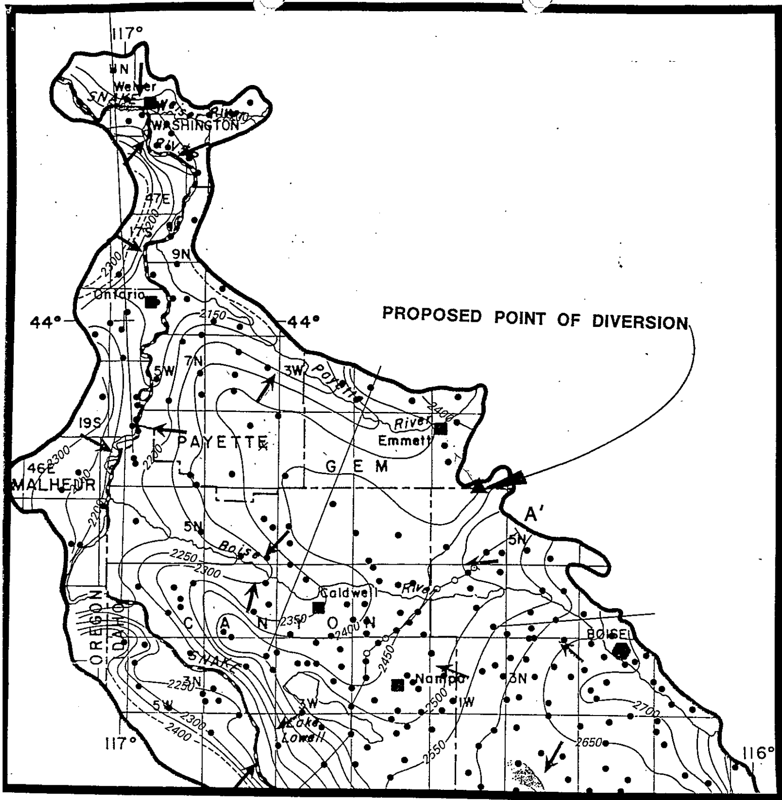
FIGURE 1 WATER-TABLE CONTOUR MAP FOR THE WESTERN SNAKE RIVER PLAIN (source: USGS Hydrologic Investigations Atlas HA-703, 1988)
