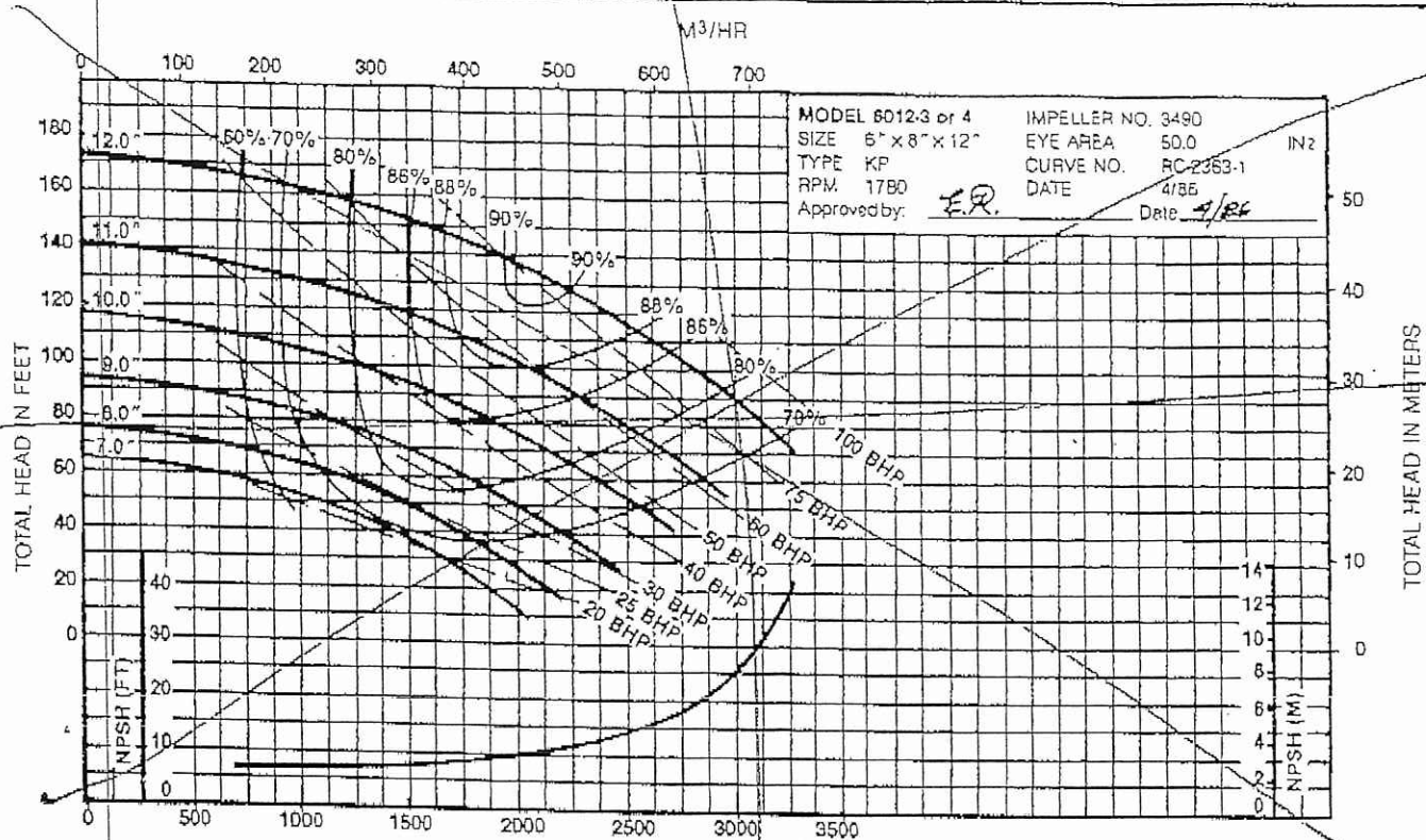
PERFORMANCE CURVES — 1750 RPM
