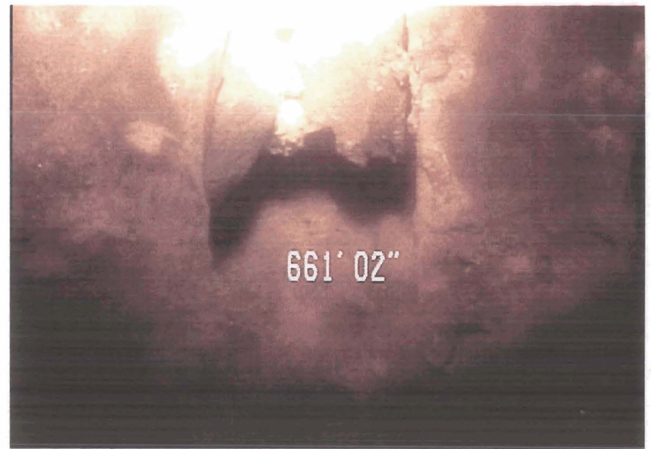
Side view still photograph of the inside wall of the ISCI Well #3 steel casing showing corrosion and natural formation sand and gravel visible through hole in the casing at ~661 feet below land surface.
