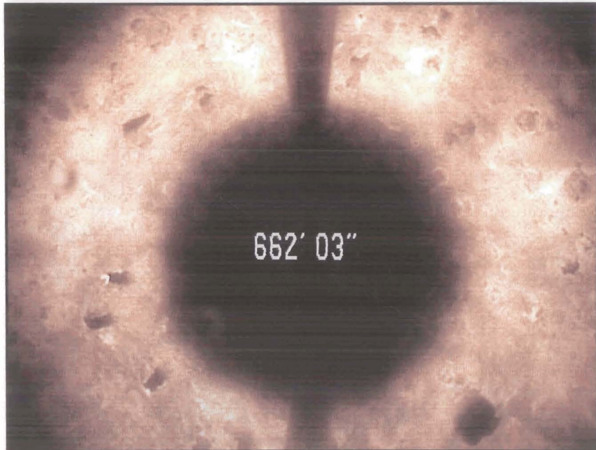
Axial (down hole) view of the corrosive pitting, holes, and cut perforations in the 42-year-old steel casing of ISCI Well #3. White numerals at center of view indicate depth below surface.
