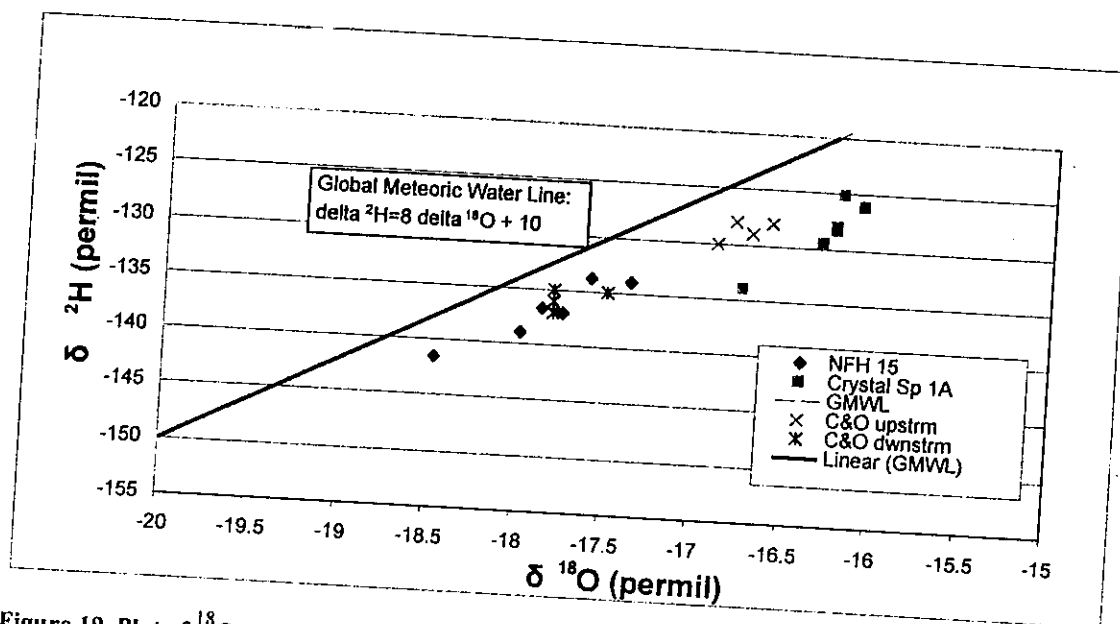
Figure 18. ^{18}\text{O} and deuterium results for National Fish Hatchery 15 (NFH 15) and Crystal Springs 1A isotope samples collected from November 2003 through March 2004.
