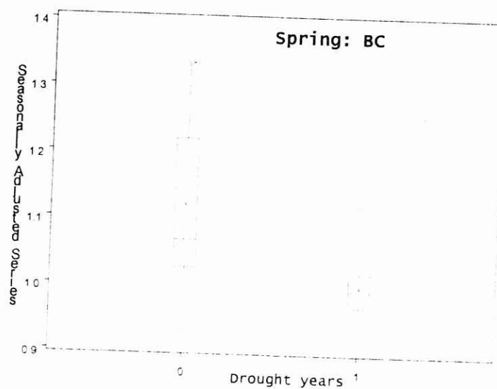
Figure 36. Box plots of nitrogen concentrations in Spring BC, comparing 1994-98 (denoted by 0) and 1999-2004 (denoted by 1) data.
