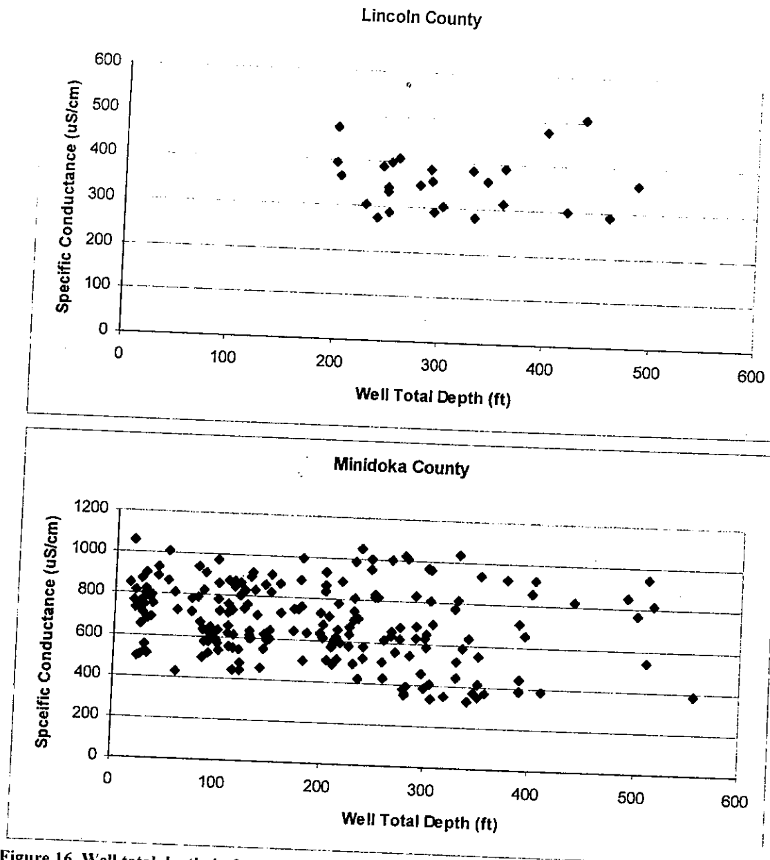
Figure 16. Well total depth, in feet versus specific conductance in \mu\text{S/cm} for Lincoln and Minidoka Counties.
