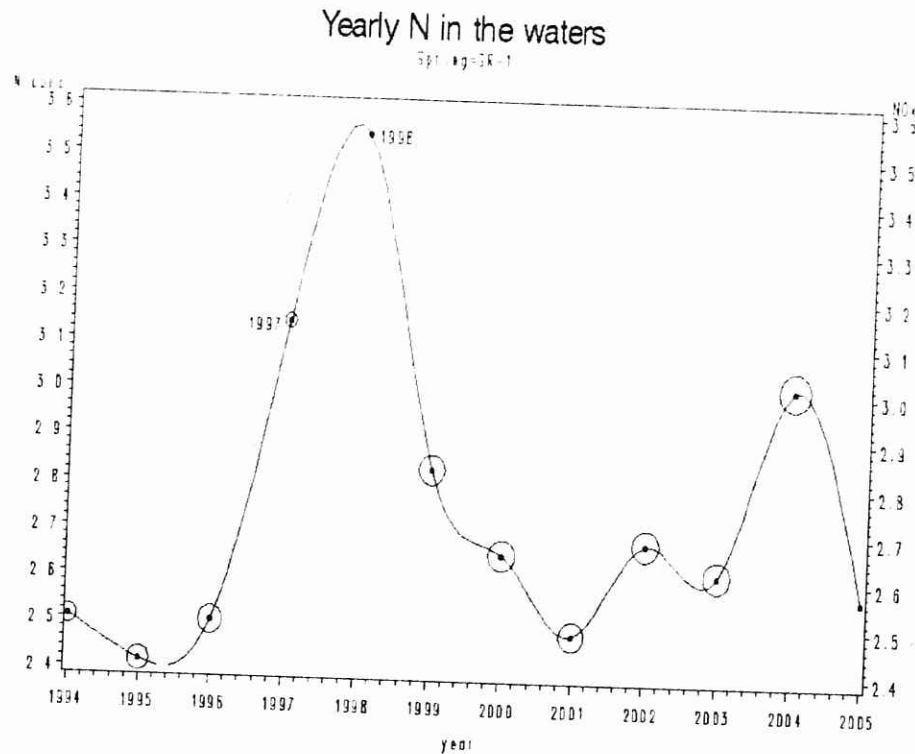
Figure 35. Variation of annual average nitrogen concentrations in spring SR-1. The bubbles represent the variability of the data: the larger the bubble, the more variable the data.
