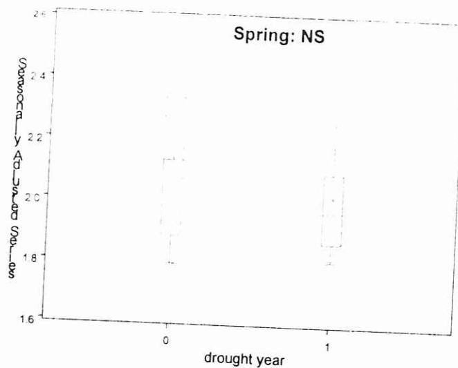
Figure 39. Box plots of nitrogen concentrations in Spring NS, comparing 1994-98 (denoted by 0) and 1999-2004 (denoted by 1) data.
