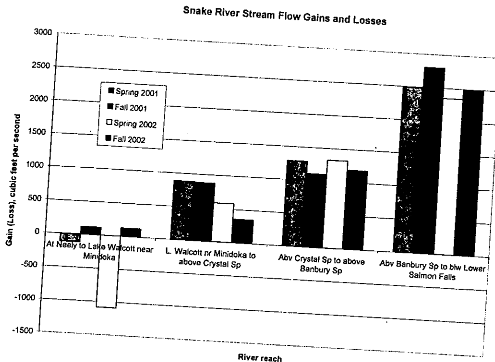
Figure 12. Snake River stream flow gains and losses from Neely to below Lower Salmon Falls (data summarized from Hortness and Vidmar, August 15, 2003).
