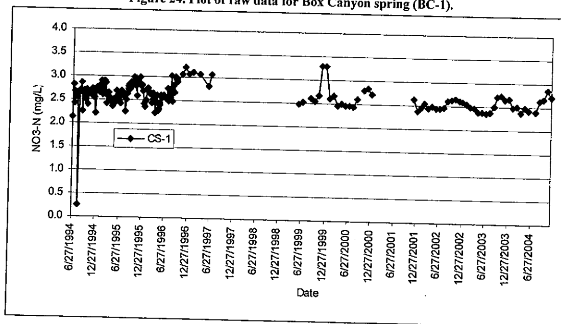
Figure 25. Plot of raw data for Crystal Springs 1 (CS-1).
