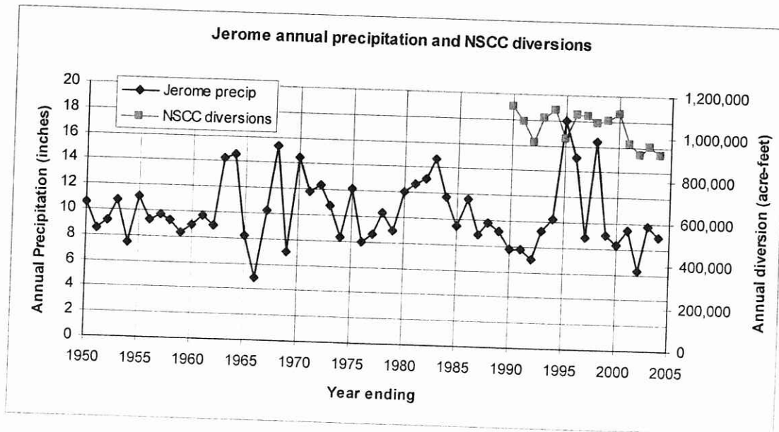
Figure 41. Annual precipitation for Jerome for the period 1950 through 2004, and North Side Canal Company (NSCC) irrigation diversions for the period 1990 through 2004.
